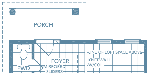
PARTIAL GROUND FLOOR B
