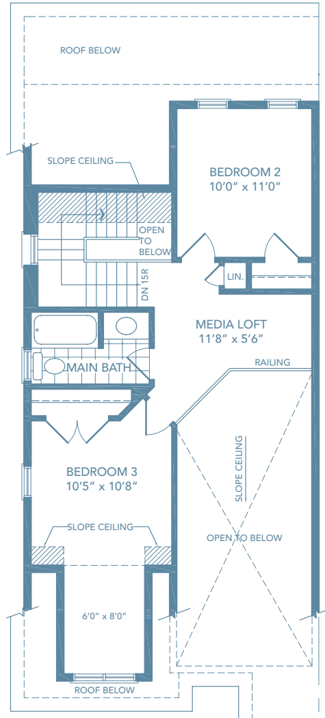
LOFT FLOOR A
