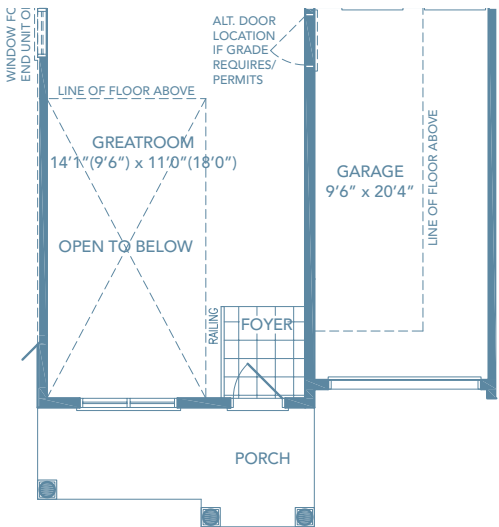
PARTIAL GROUND FLOOR B
