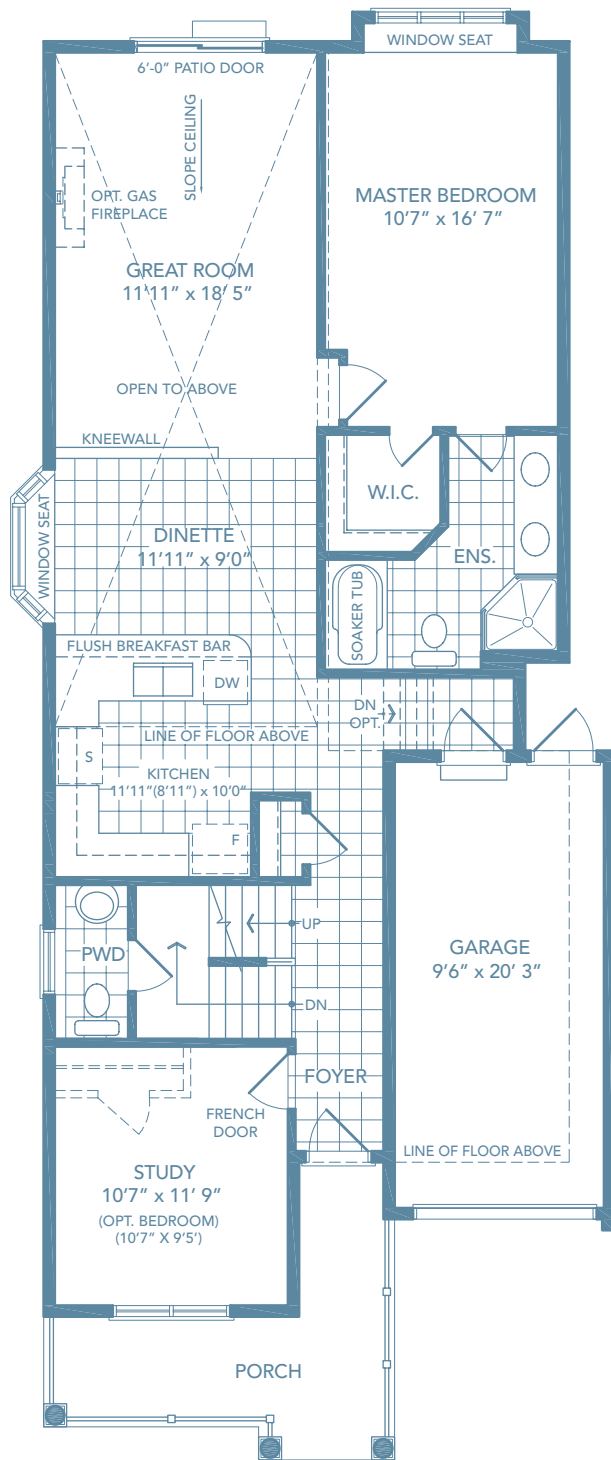
GROUND FLOOR A & B END UNIT
